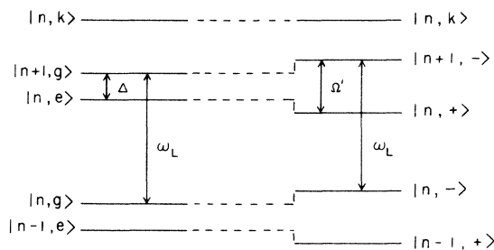
FIG. 1. Energy levels of the bare system plus the free laser field are represented by the diagram on the left-hand side. The detuning \Delta is taken positive. The number of photons in the laser mode is indicated by n . If the dipole coupling -\mu \cdot \mathbf{E} is included, a new diagonalization yields the dressed energy-level system on the right-hand side. The level separations \Delta and \omega_L in the bare system now become \Omega' and \omega_L , where \Omega' is always larger than \Delta due to \Omega^2 \neq 0 . This is the ac-Stark shift (Ref. 27). The state |k\rangle , which is not coupled to another level by the laser, remains unaltered. In general, we suppress the quantum number n and represent the dressed atom as an infinite ladder of states |\pm\rangle , which is the famous Jaynes-Cummings model for the interaction of a two-level system with a strong radiation field (Ref. 28).
