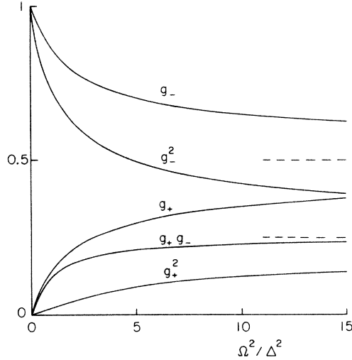
FIG. 3. Optical factors in the transition rates as a function of \Omega^2/\Delta^2 . For strong fields or small detunings, both g_+ and g_- tend to their asymptotic value of \frac{1}{2} , which is the upper dotted line, and g_+^2 , g_-^2 , and g_+g_- will approach \frac{1}{4} in this limit. For weak fields or large detunings, we have g_- = g_-^2 = 1 and g_+ = g_+^2 = g_+g_- = 0 . For increasing field strengths, the g_-^2 transition will diminish very strongly, in favor of the other three processes between the |\pm\rangle doublets.
