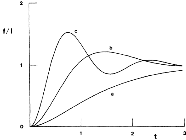
FIG. 1. Plot of the two-photon correlation function f_\eta(t)/I_\eta in the low-intensity limit. Time and frequencies are given in units of 1/A_f and A_f , respectively, and the distance between the atom and the surface h is in units of an optical wavelength 2\pi c/\omega_0 . In this figure we take h=0.2 , \lambda=0.5 , and linear polarization. Curves a , b , and c illustrate the dependence on the detuning, with \Delta=0 , 2 , and 4 , respectively. Notice that f(t) can become larger than f(\infty) , which implies an enhancement for the detection of a photon at time t after the detection of a photon at time zero, in comparison with the uncorrelated detection probability I .
