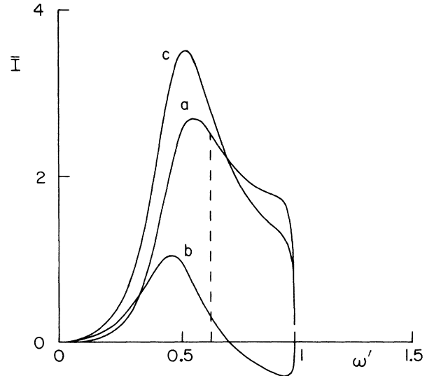
FIG. 2. Curves a and b are \bar{I}(\omega)_{\text{reg}} and \bar{I}(\omega)_{\text{in}} , respectively, for the same parameters as in Fig. 1. Their sum, curve c , is \bar{I}(\omega) , which is calculated with the present theory. Comparison of curves a and c shows the significance of the improvement. Note also the considerable red shift of the line with respect to the resonance frequency \omega_0 .
