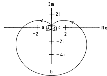
FIG. 9. Polar plot of P_s as a function of \omega_a/\bar{\omega} in the complex plane, and for the same parameters as in Fig. 7. The arrowheads indicate the direction of increasing frequency, and points a , b , and c correspond to \omega_a/\bar{\omega}=0.993 , 1.000 , and 1.007 , respectively. These points correspond to the central peak and the two sidebands in Fig. 7. The polar angle equals the phase shift upon reflection.
