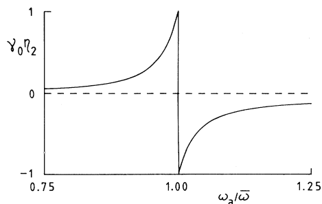
FIG. 3. Plot of \gamma_0\eta_2 as a function of \omega_a/\bar{\omega} for \epsilon=1 and \gamma_0=0.1 . At resonance this parameter is discontinuous, with |\gamma_0\eta_2|=1 , and far off resonance it goes to zero.
