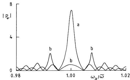
FIG. 7. Curves a and b represent |P_s| and |P_p| , respectively, as a function of \omega_a/\bar{\omega} . The parameters are \epsilon=1 , \gamma=0.01 , d=105 , and \kappa_{||}=1/\sqrt{2} . The peak heights are different for s and p waves, and the maxima appear at different frequencies. The peak at resonance for p waves is weaker than two of the sidebands.
