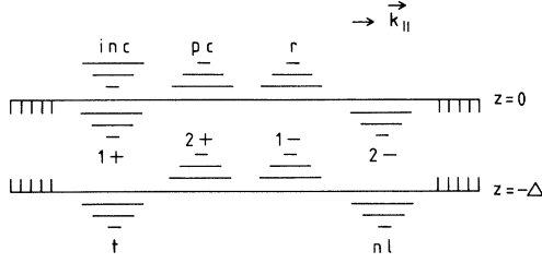
FIG. 5. Same as Fig. 4 but for evanescent waves. The \omega_a waves travel into the direction of \vec{k}_{||} , whereas the \omega_b waves travel to the left. Two waves in a pair travel in opposite directions but decay in the same direction.
