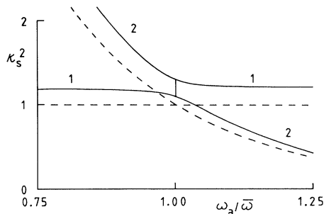
FIG. 2. This figure shows the two branches of the dispersion relation for s-polarized waves, as given by Eq. (7.5). Plotted is the square of the wave vector versus the frequency in units of the pump frequency, for \epsilon=1 and \gamma_0=0.1 . The dashed lines indicate the corresponding relations for a dielectric ( \gamma_0=0 ).
