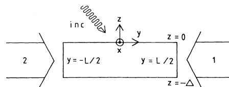
FIG. 1. Schematic setup of a PC operating by FWM. The crystal is bounded by the z=0 and z=-\Delta planes and irradiated by two strong laser beams, propagating parallel to the xy plane, and they illuminate the medium at y=L/2 and y=-L/2 . Also shown is the weak incident field which will be phase conjugated by the PC.
