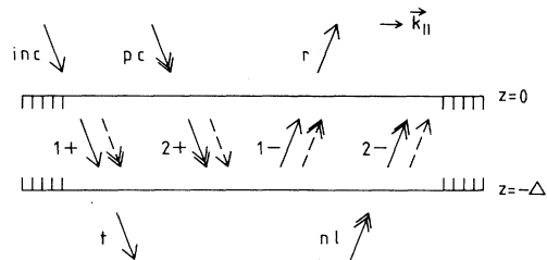
FIG. 4. Schematic representation of the various traveling waves which can be excited simultaneously by the incident field. The solid arrows indicate a principal wave, which can either be an \omega_a wave (for 1\pm ) or an \omega_b wave (for 2\pm ), and the broken arrows represent the waves which are coupled to the principal waves via the nonlinear interaction. A double arrowhead indicates a wave vector of an \omega_b wave, which travel into the direction opposite the wave vector (because \omega_b is negative).
