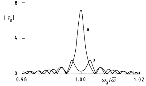
FIG. 8. Plot of |P_s| versus \omega_a/\bar{\omega} for two values of the layer thickness d . Curves a and b correspond to d=105 and d=150 , respectively, and the other parameters are \epsilon=1 , \gamma=0.01 , and \kappa_{||}=1/\sqrt{2} . Curve b shows that |P_s| can have a minimum at resonance.
