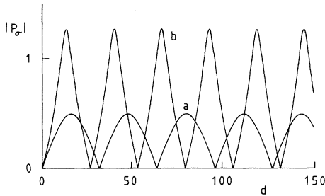
FIG. 10. Curves a and b give |P_s| and |P_p| , respectively, as a function of the layer thickness d . The parameters are taken to be \omega_a/\bar{\omega}=1.01 , \epsilon=1 , \gamma=0.01 , and \theta_i=45^\circ . The peaks appear to be equidistant, as they should according to Eqs. (13.9), (13.11), and (13.12).
