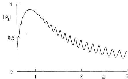
FIG. 11. Plot of |P_s| versus the dielectric constant \epsilon , for \omega_a/\bar{\omega}=0.985 , \gamma=0.03 , d=10 , and \kappa_{||}=1/\sqrt{2} . The maximum phase-conjugate reflectivity occurs around \epsilon=1 . For larger values of \epsilon the reflectivity decreases rapidly, and in an oscillatory way. At \epsilon=0.5 we have \epsilon=\kappa_{||}^2 , which implies \kappa_{as}=\kappa_{bs}=0 . At this point the waves inside the medium become evanescent, and the phase-conjugate signal disappears.
