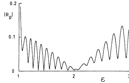
FIG. 12. Plot of the reflection coefficient |R_p| as a function of the dielectric constant, and for \omega_a/\bar{\omega}=0.985 , \gamma=0.05 , d=10 , and \kappa_{||}=0.819(\theta_i=55^\circ) . For \epsilon=1 the reflectivity is not identically zero, which is due to the nonlinear interaction ( \gamma \neq 0 ). Similarly, at \epsilon=2 we have \epsilon=\tan^2\theta_i , so that \theta_i equals the Brewster angle. The linear interaction would then give R_p=0 , but for \gamma \neq 0 there is a residual reflection into the specular direction.
