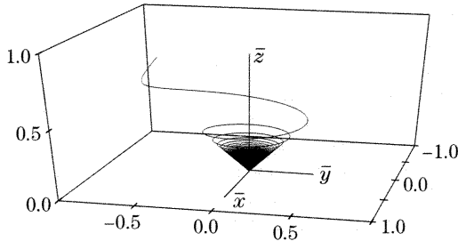
Fig. 1. Typical field line of the Poynting vector for the radiation emitted by an electric dipole with \beta = 1 , located at the origin of coordinates. The field line lies on a cone (of 45^\circ with the z axis for this example). Near the source, the field line rotates numerous times around the z axis and this gives the vortex structure in the near-field emission pattern. We use dimensionless variables \bar{x} = \omega x/c , etc., so that a distance of 2\pi corresponds to one optical wavelength.
