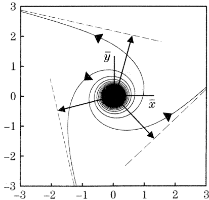
Fig. 2. Three field lines in the xy plane ( \theta_O = \pi/2 ) for a circular dipole ( \beta = 1 ). The field lines approach asymptotically the dashed lines, corresponding to various values of the observation angle \phi_O .
