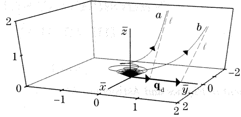
Fig. 3. Field lines for \beta = 1 , \phi_O = \pi . Curves a and b correspond to observation angles \theta_O = \pi/6 and \theta_O = \pi/3 , respectively. Far away from the source, the field lines approach straight lines indicated by \ell . When viewed from the far field, a curved field line is indistinguishable from the asymptotic line \ell , and this gives rise to an apparent displacement of the source. The image point in the xy plane is the intersection between \ell and the xy plane, and the location of this point is represented by the displacement vector \mathbf{q}_d .
