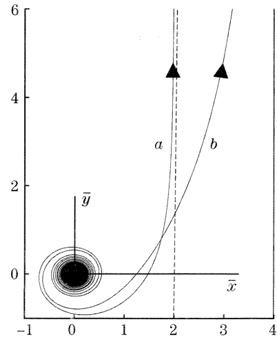
Fig. 4. Field lines for \theta_O = \pi/2 and \phi_O = \pi/2 . Curves a and b correspond to \beta = 1 and \beta = 0.5 , respectively. The dashed lines are the asymptotes. The displacement vectors are along the x axis, and their magnitudes are q_d = 2 and q_d = 4 , respectively.
